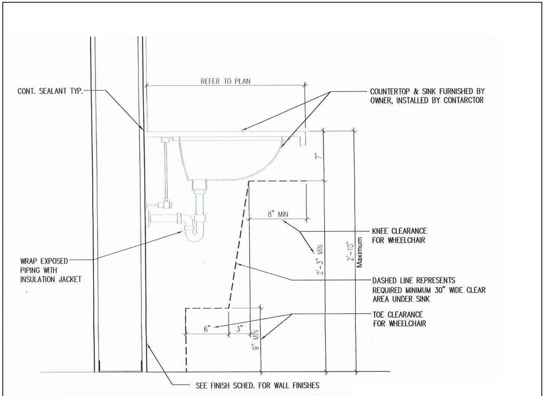
TYPICAL COUNTER @ ACCESSIBLE SINK
