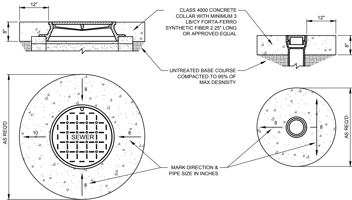
SINGLE ITEM CONCRETE COLLAR
