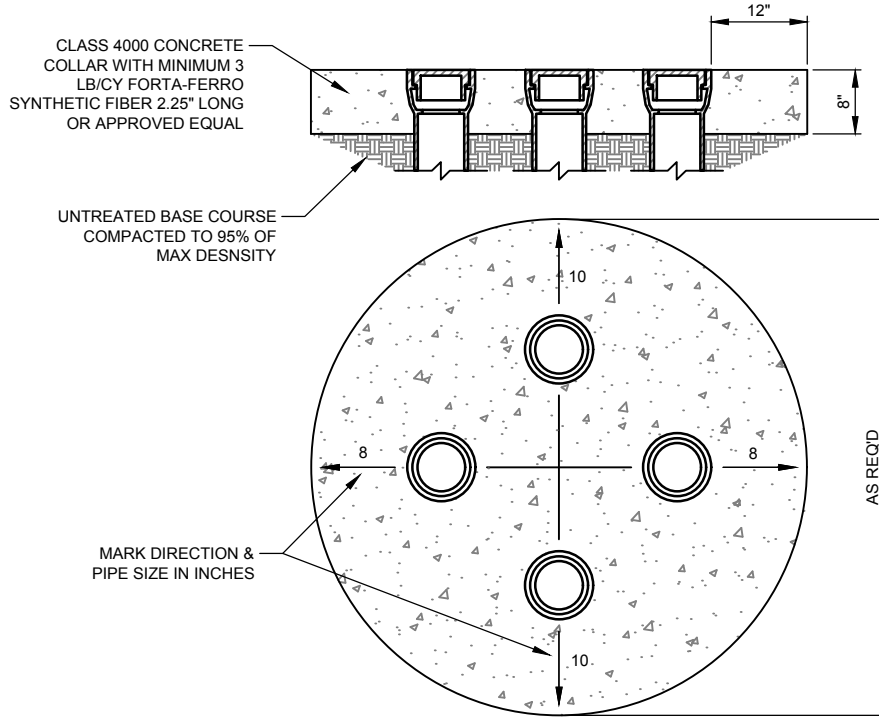
MULTIPLE ITEM CONCRETE COLLAR
